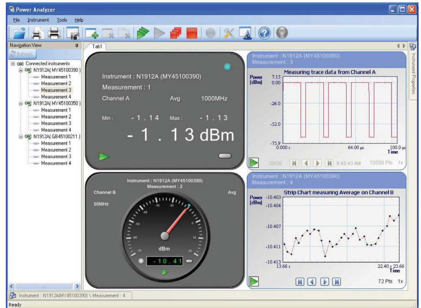
Figure 19. N1918A Power Analyzer
