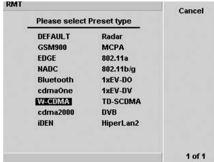
Figure 10. Pre-defined test setups
