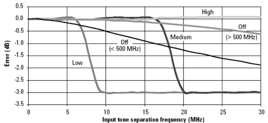
Figure 7. N192XA Error in peak-to-average measurements for a two-tone input (High, Medium and Low or Off video bandwidth)
